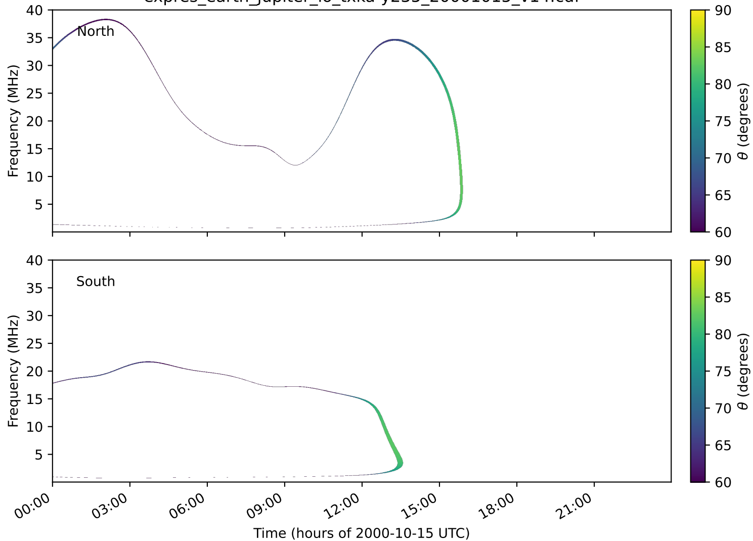
expres_earth_jupiter_io_txka-y235_20001015_v14.cdf
