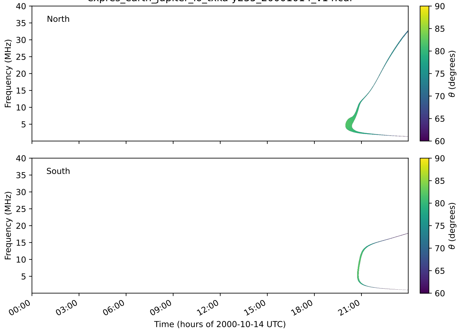
expres_earth_jupiter_io_txka-y235_20001014_v14.cdf
