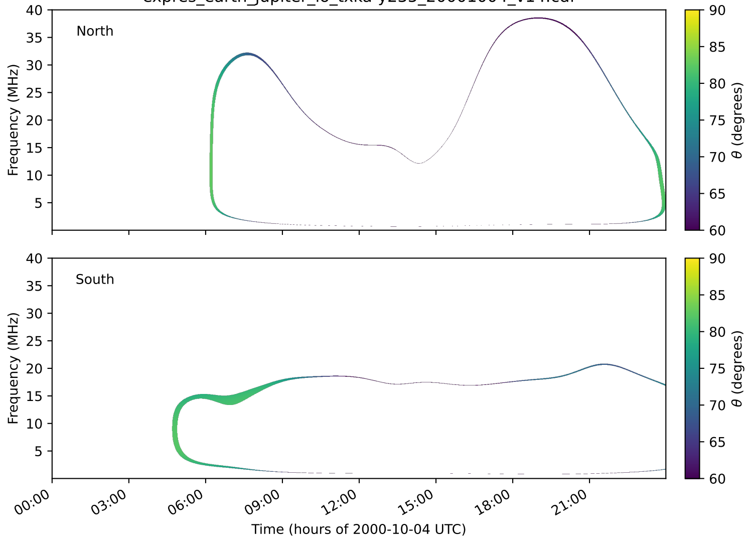
expres_earth_jupiter_io_txka-y235_20001004_v14.cdf
