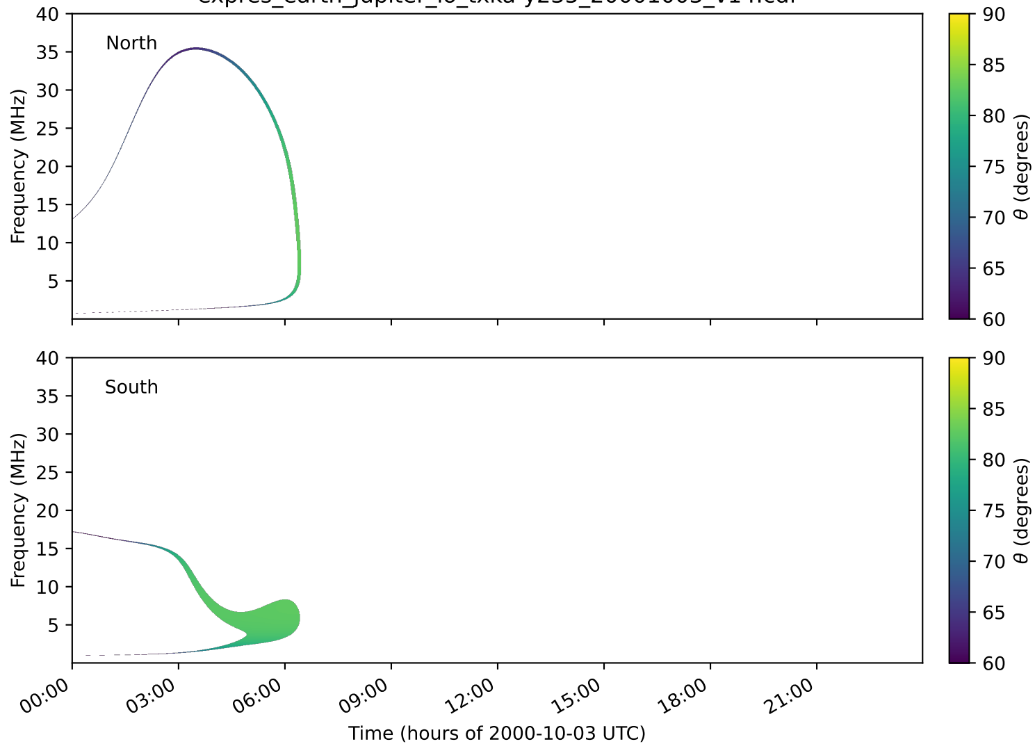
expres_earth_jupiter_io_txka-y235_20001003_v14.cdf
