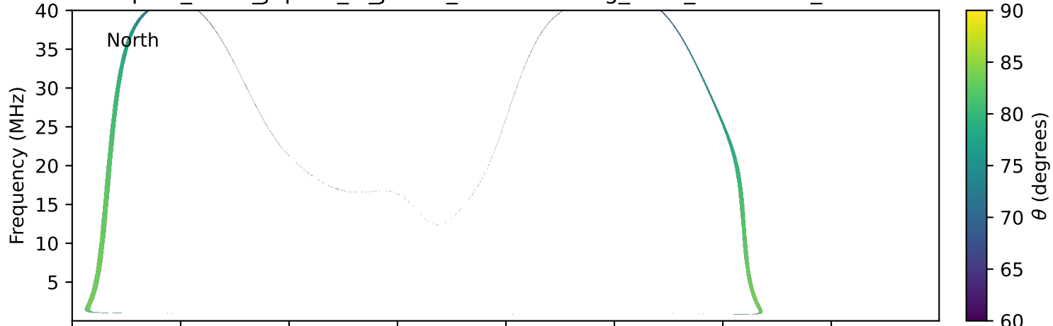
expres_earth_jupiter_io_jrm33_lossc-wid1deg_3kev_20001029_v11.cdf
