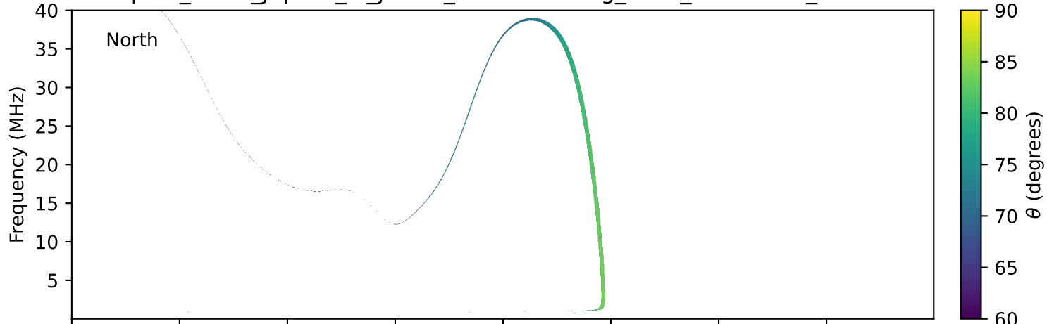
expres_earth_jupiter_io_jrm33_lossc-wid1deg_3kev_20001008_v11.cdf
