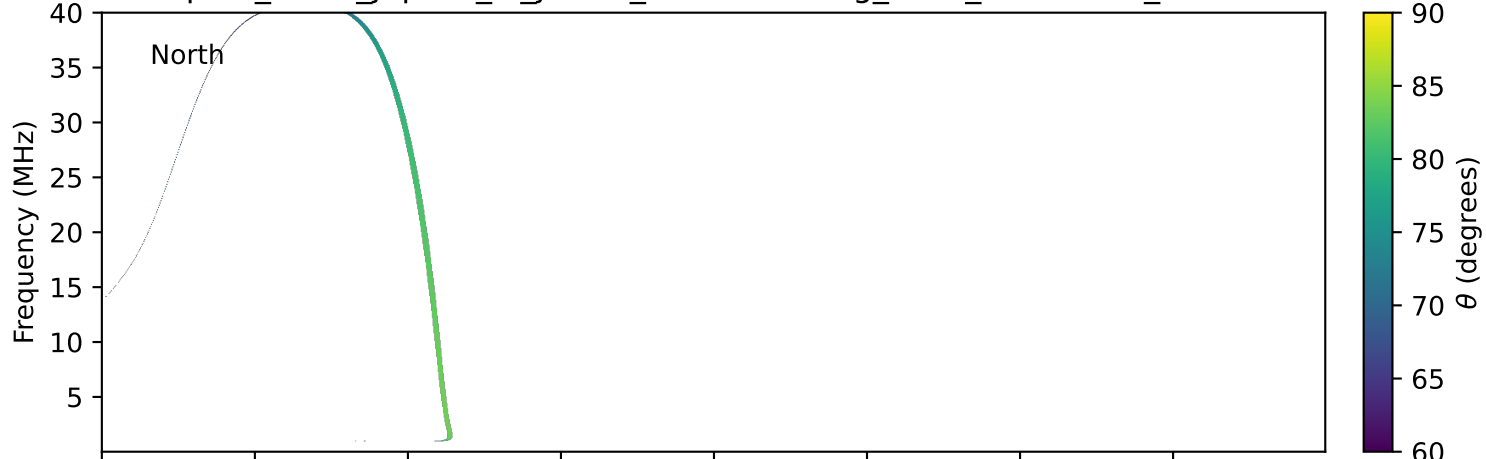
expres_earth_jupiter_io_jrm33_lossc-wid1deg_3kev_20001003_v11.cdf
