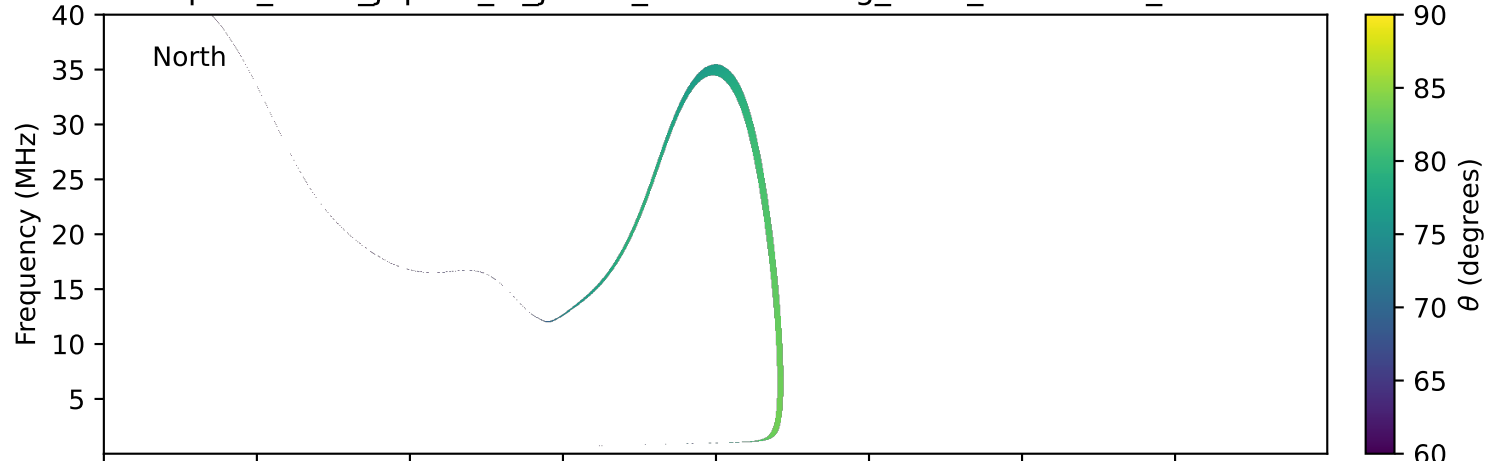
expres_earth_jupiter_io_jrm33_lossc-wid1deg_3kev_20001001_v11.cdf
