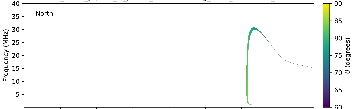
expres_earth_jupiter_io_jrm09_lossc-wid1deg_3kev_20001030_v11.cdf
