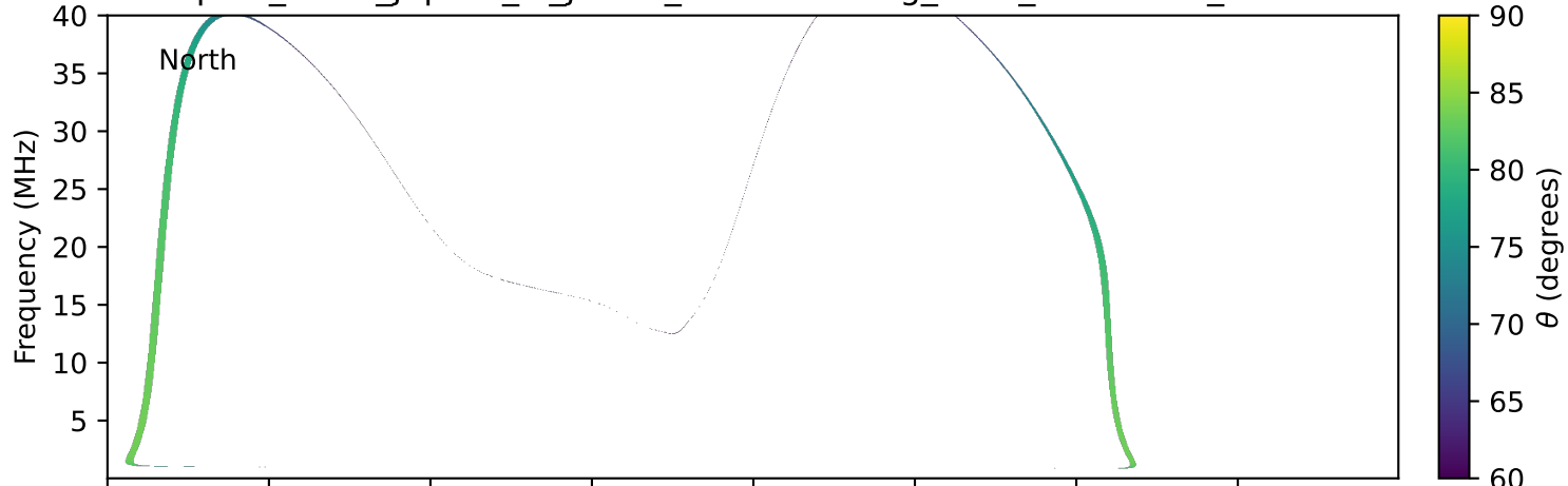
expres_earth_jupiter_io_jrm09_lossc-wid1deg_3kev_20001029_v11.cdf
