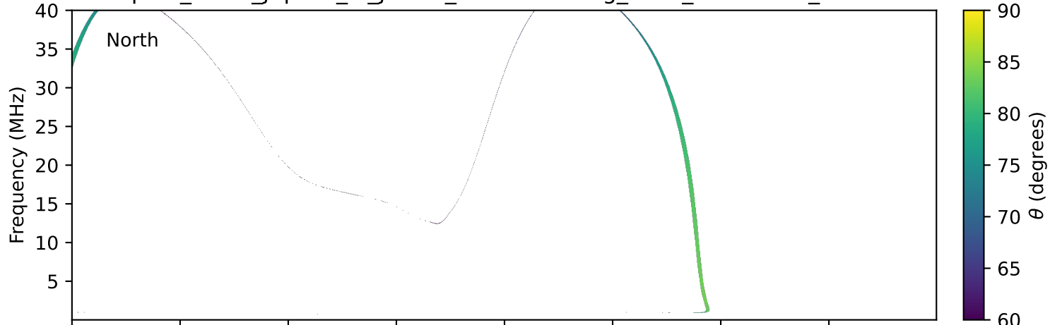
expres_earth_jupiter_io_jrm09_lossc-wid1deg_3kev_20001022_v11.cdf
