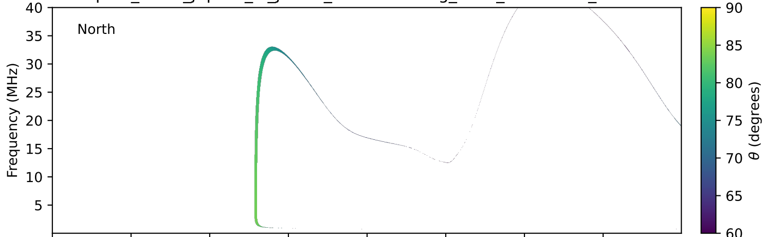
expres_earth_jupiter_io_jrm09_lossc-wid1deg_3kev_20001011_v11.cdf
