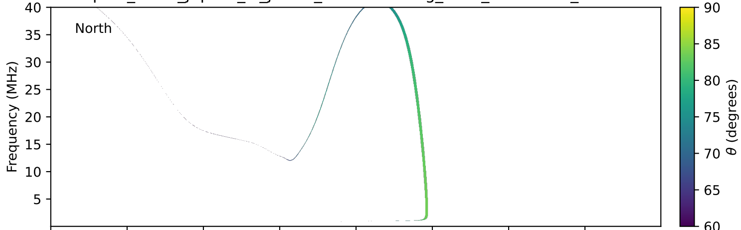
expres_earth_jupiter_io_jrm09_lossc-wid1deg_3kev_20001008_v11.cdf
