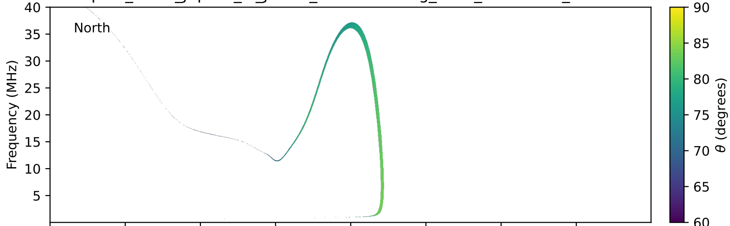
expres_earth_jupiter_io_jrm09_lossc-wid1deg_3kev_20001001_v11.cdf
