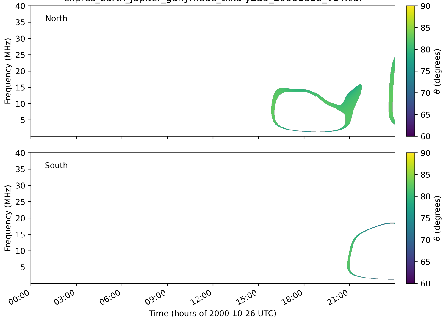
expres_earth_jupiter_ganymede_txka-y235_20001026_v14.cdf
