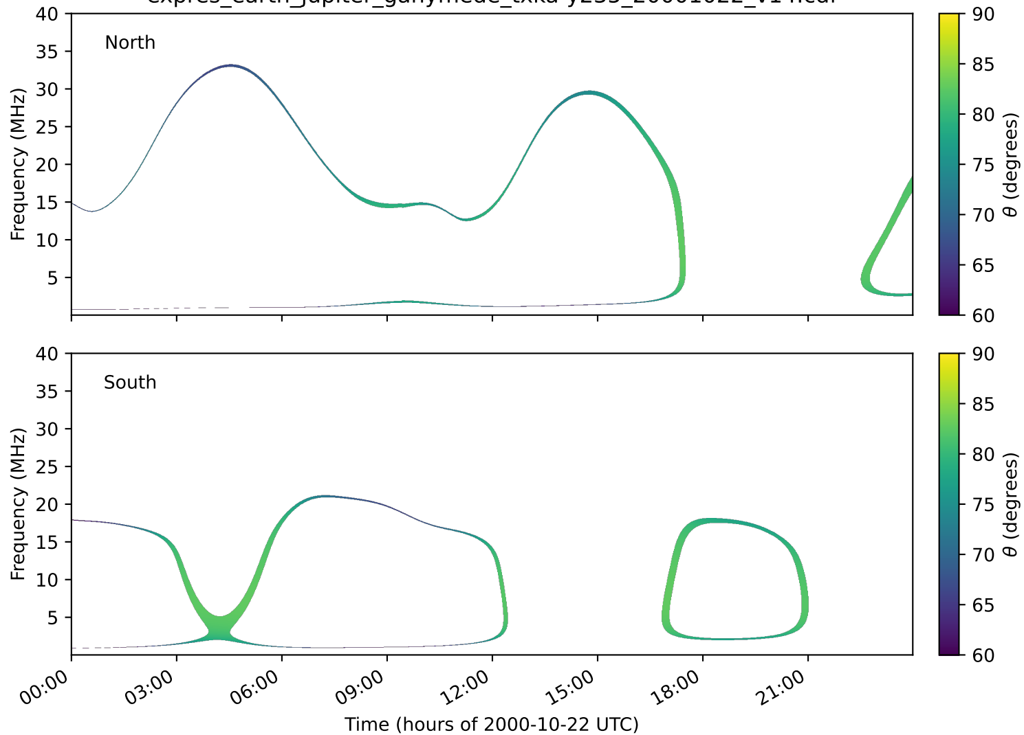
expres_earth_jupiter_ganymede_txka-y235_20001022_v14.cdf
