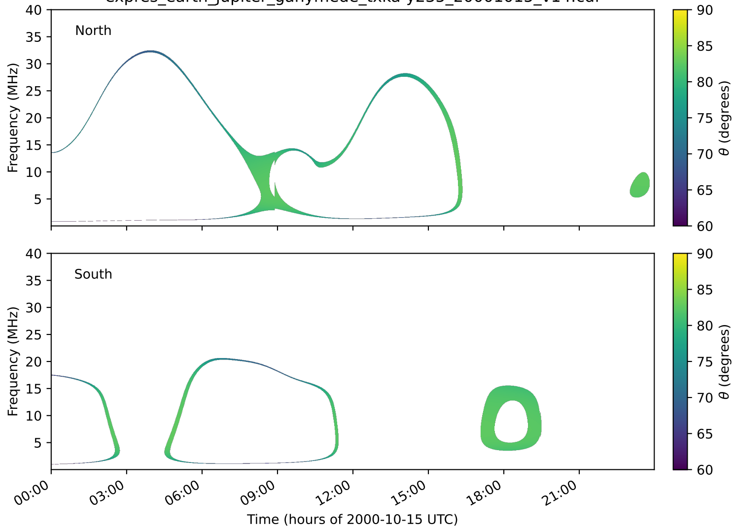
expres_earth_jupiter_ganymede_txka-y235_20001015_v14.cdf
