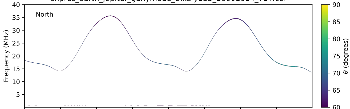
expres_earth_jupiter_ganymede_txka-y235_20001014_v14.cdf
