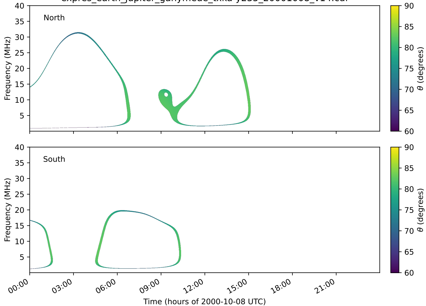
expres_earth_jupiter_ganymede_txka-y235_20001008_v14.cdf
