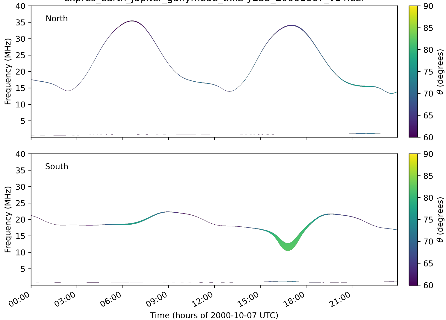
expres_earth_jupiter_ganymede_txka-y235_20001007_v14.cdf
