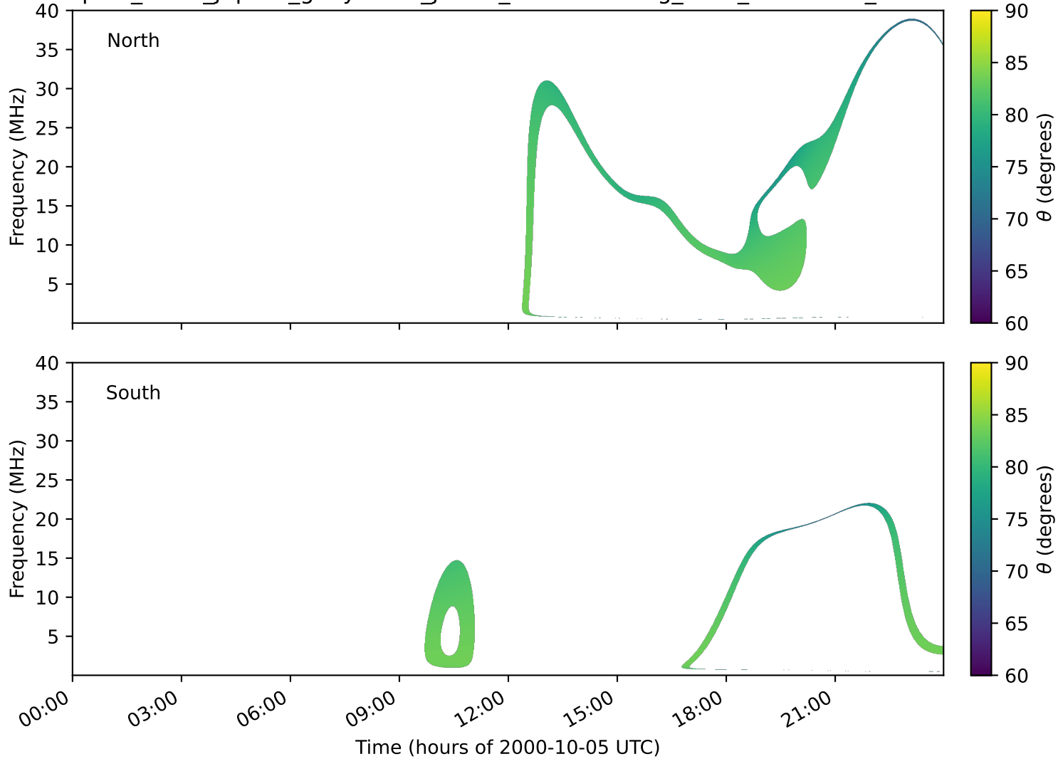
expres_earth_jupiter_ganymede_jrm33_lossc-wid1deg_3kev_20001005_v11.cdf
