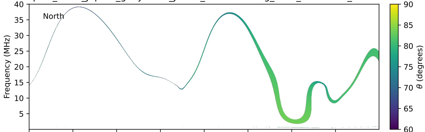
expres_earth_jupiter_ganymede_jrm09_lossc-wid1deg_3kev_20001015_v11.cdf
