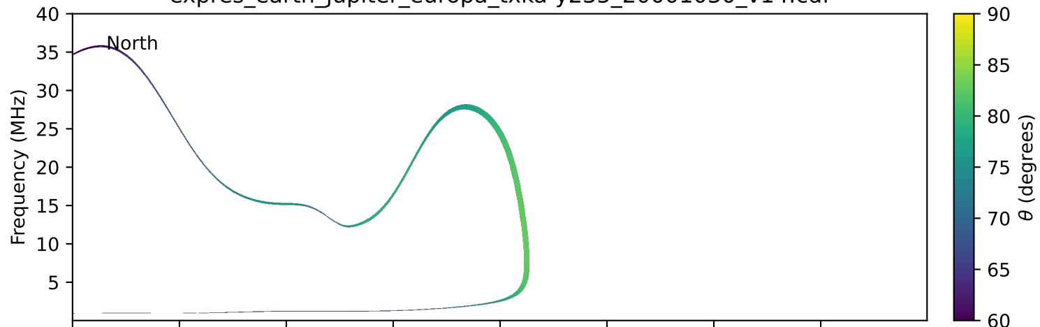
expres_earth_jupiter_europa_txka-y235_20001030_v14.cdf
