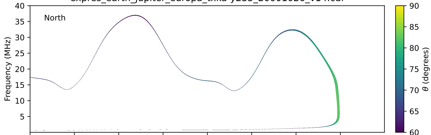
expres_earth_jupiter_europa_txka-y235_20001026_v14.cdf
