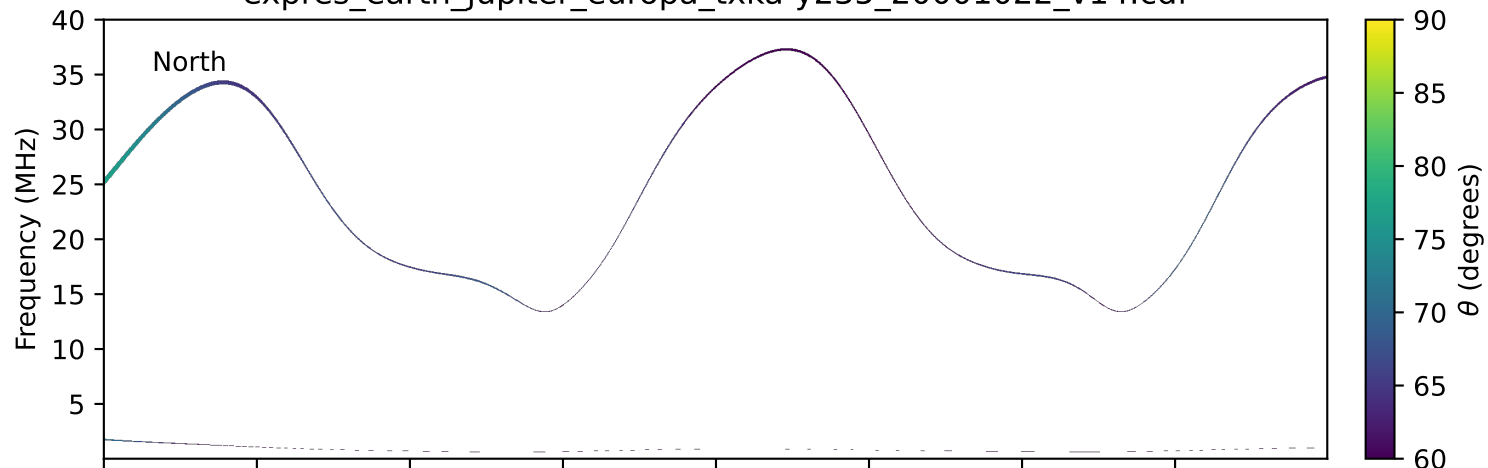
expres_earth_jupiter_europa_txka-y235_20001022_v14.cdf
