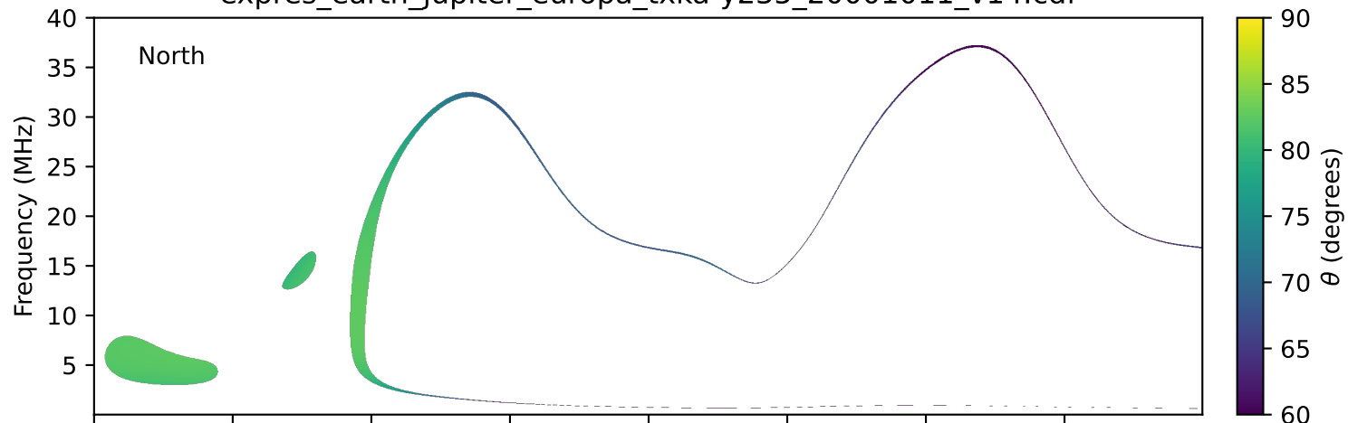
expres_earth_jupiter_europa_txka-y235_20001011_v14.cdf
