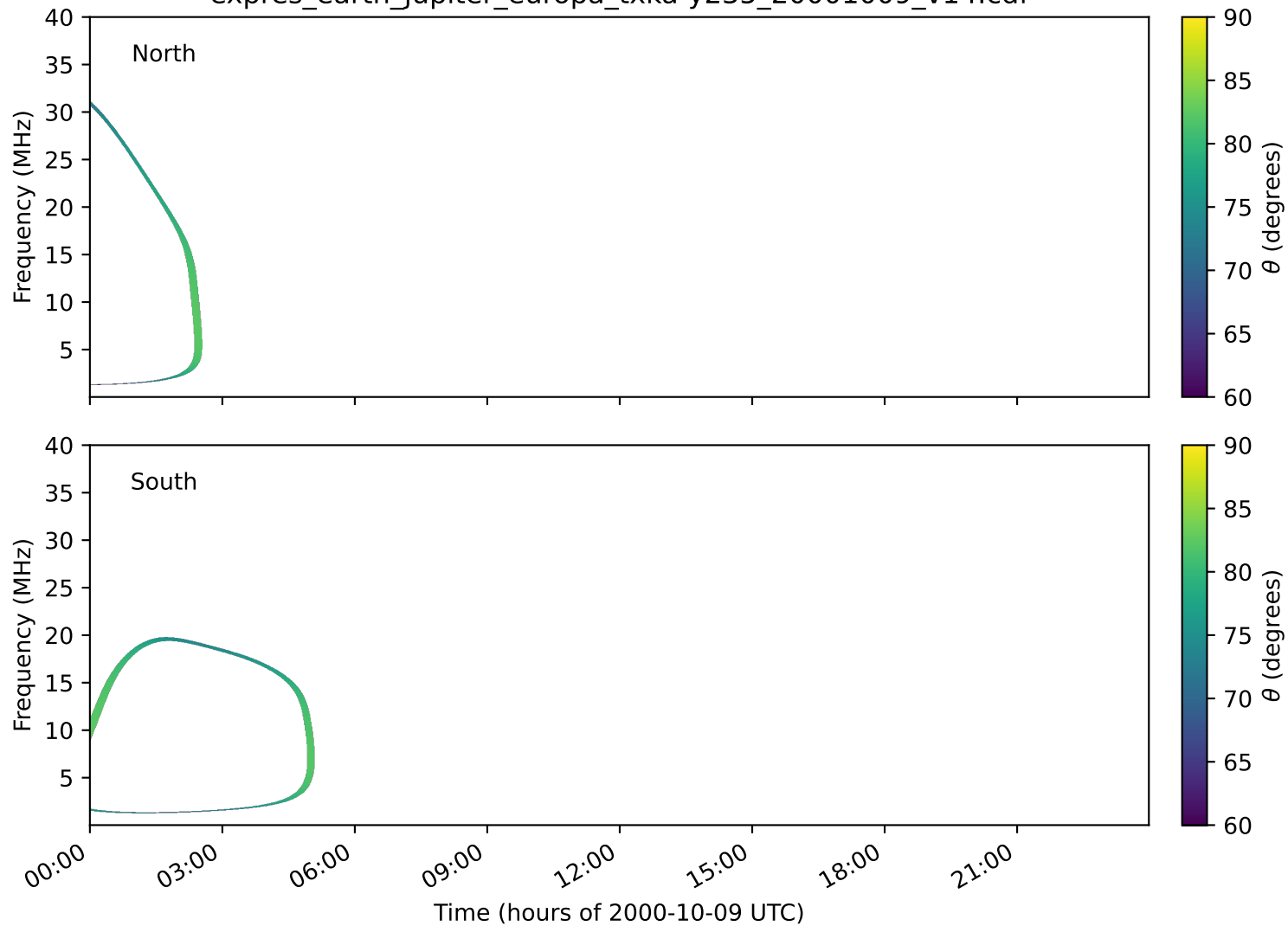
expres_earth_jupiter_europa_txka-y235_20001009_v14.cdf
