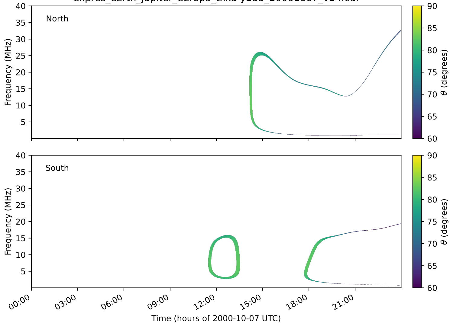
expres_earth_jupiter_europa_txka-y235_20001007_v14.cdf
