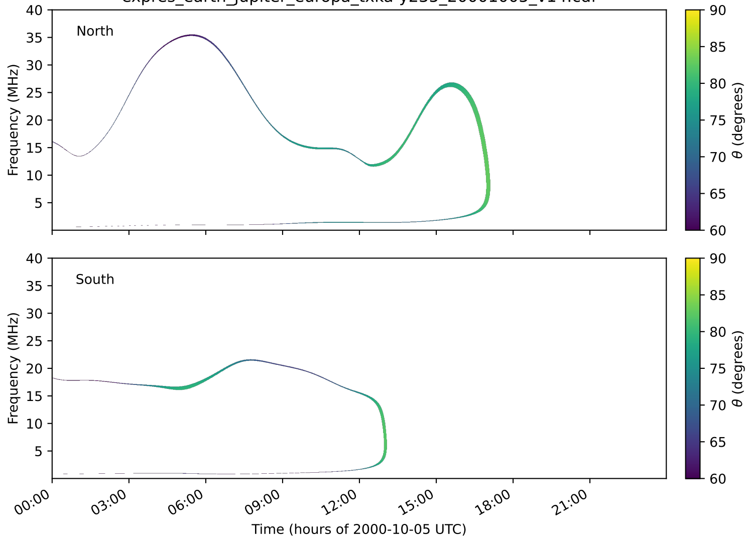
expres_earth_jupiter_europa_txka-y235_20001005_v14.cdf
