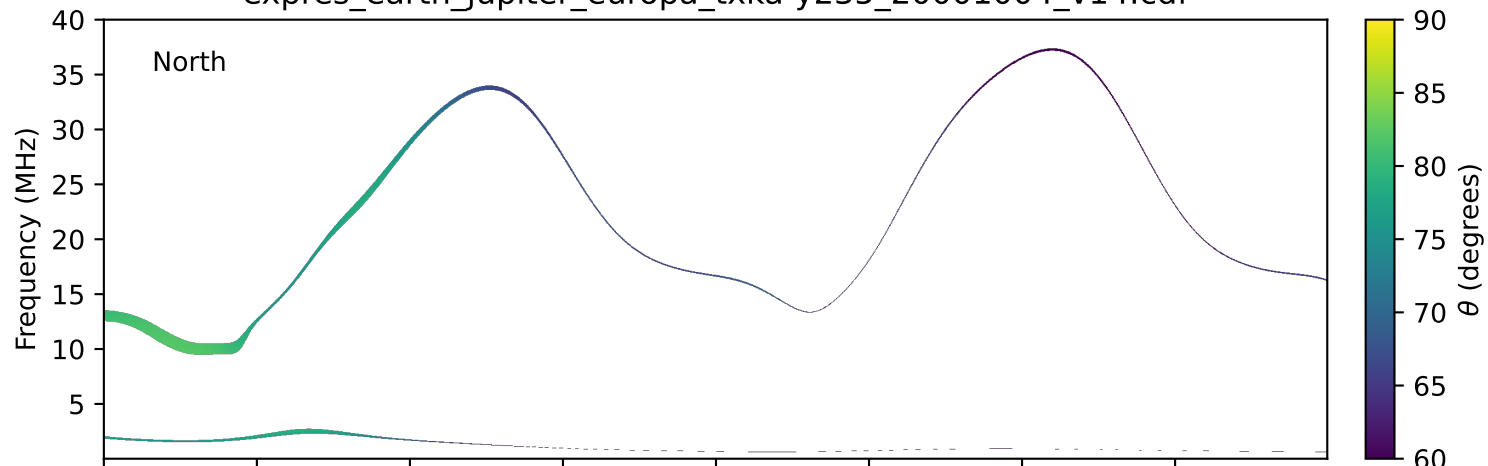
expres_earth_jupiter_europa_txka-y235_20001004_v14.cdf
