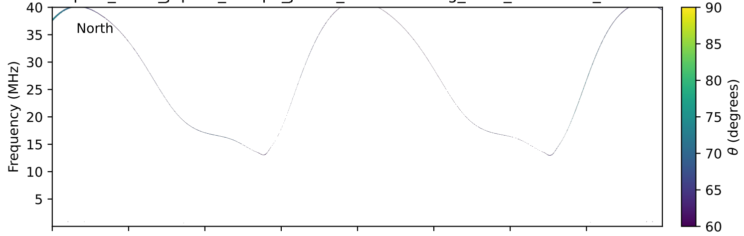
expres_earth_jupiter_europa_jrm09_lossc-wid1deg_3kev_20001015_v11.cdf
