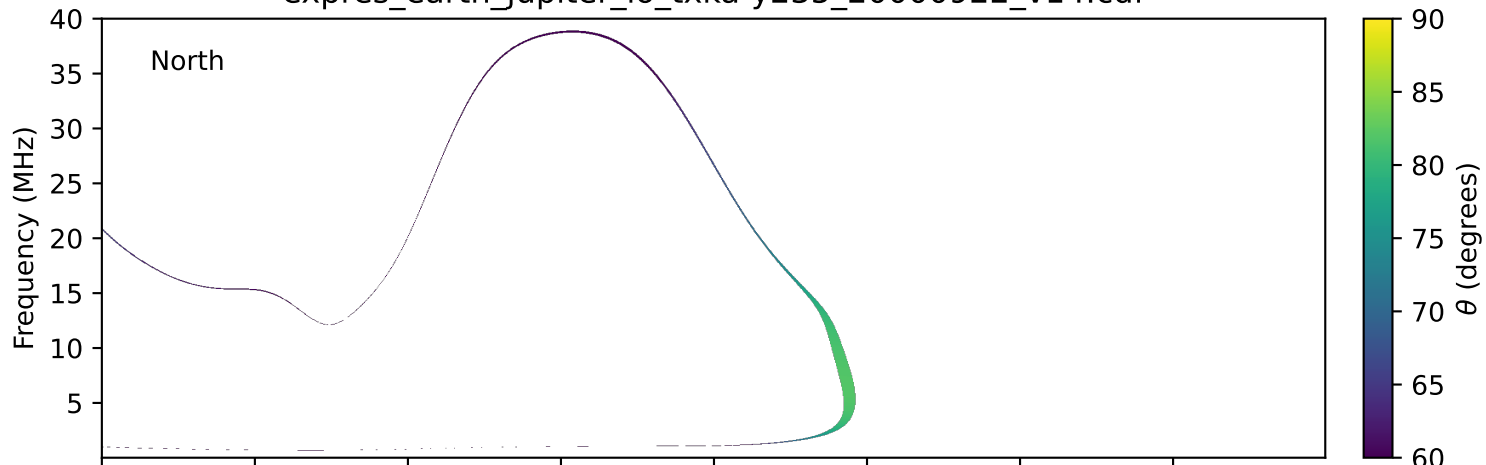
expres_earth_jupiter_io_txka-y235_20000922_v14.cdf
