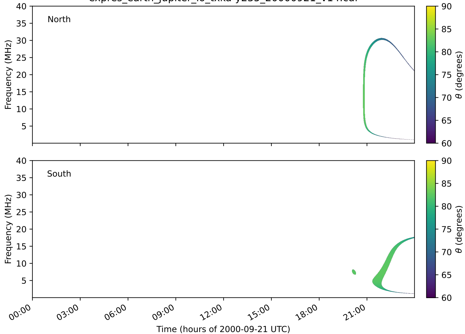
expres_earth_jupiter_io_txka-y235_20000921_v14.cdf
