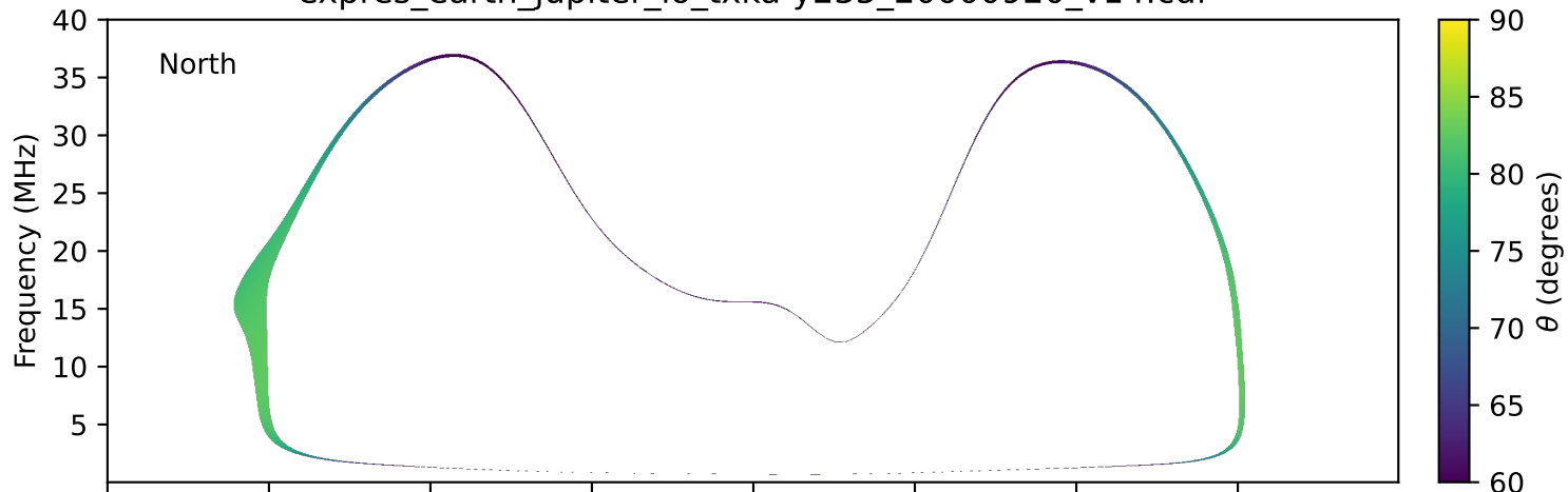
expres_earth_jupiter_io_txka-y235_20000920_v14.cdf
