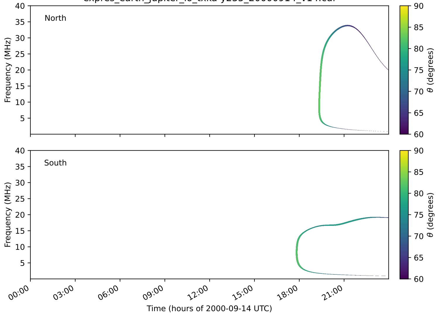
expres_earth_jupiter_io_txka-y235_20000914_v14.cdf
