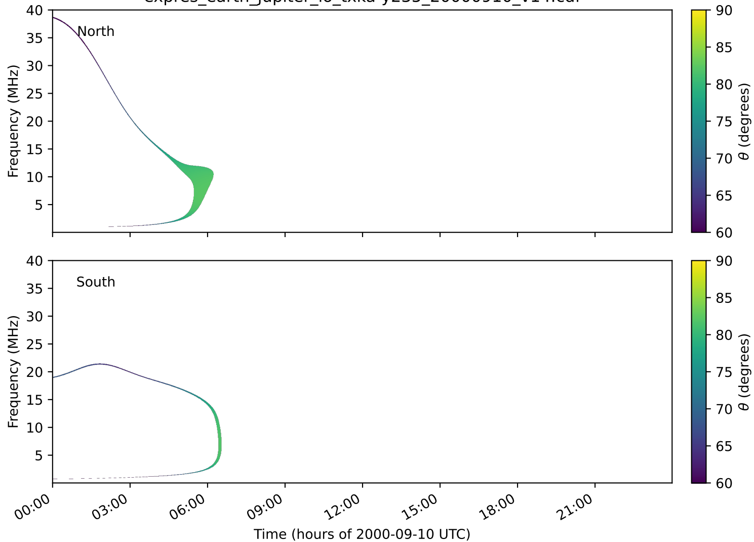
expres_earth_jupiter_io_txka-y235_20000910_v14.cdf
