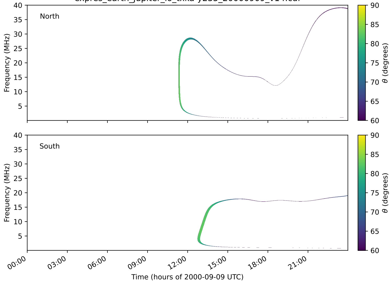
expres_earth_jupiter_io_txka-y235_20000909_v14.cdf
