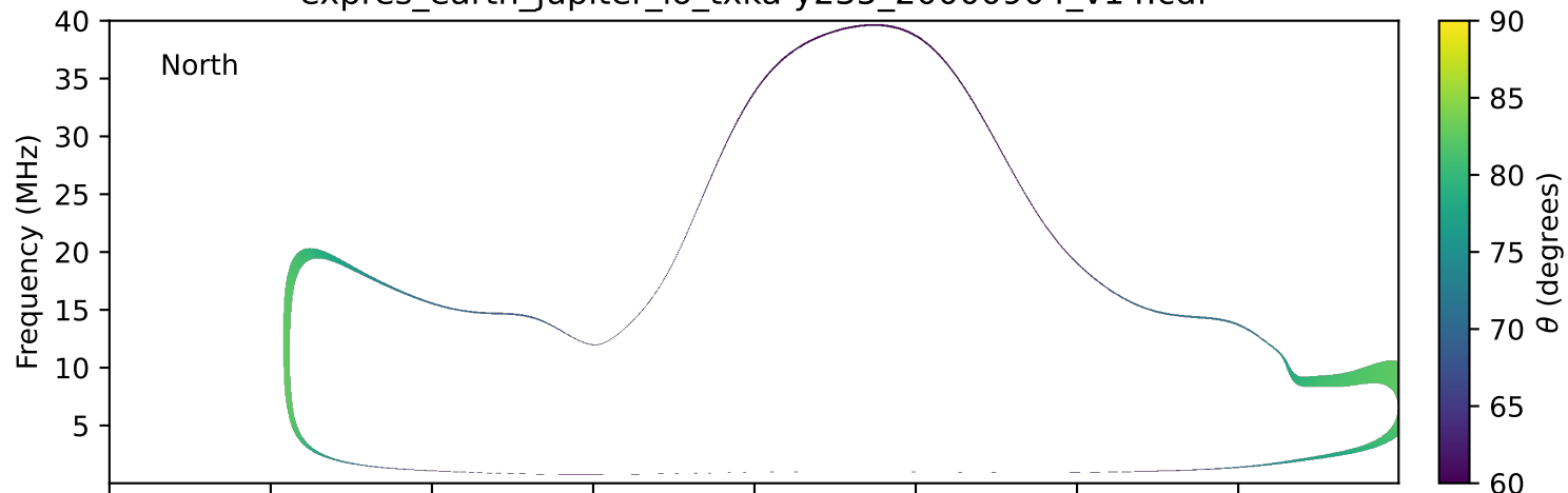
expres_earth_jupiter_io_txka-y235_20000904_v14.cdf
