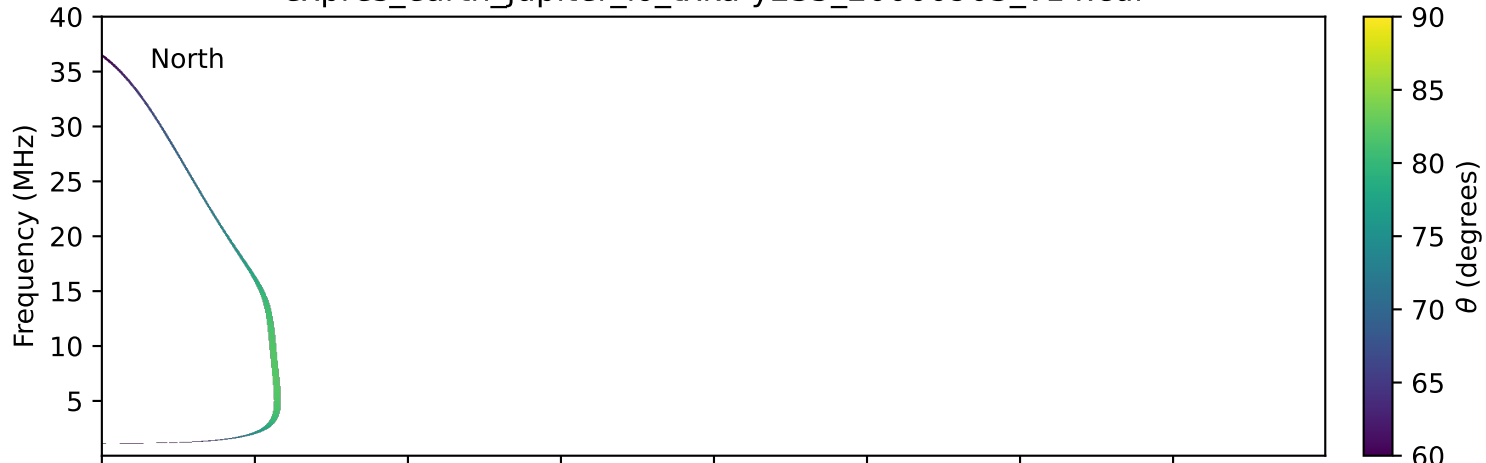
expres_earth_jupiter_io_txka-y235_20000903_v14.cdf
