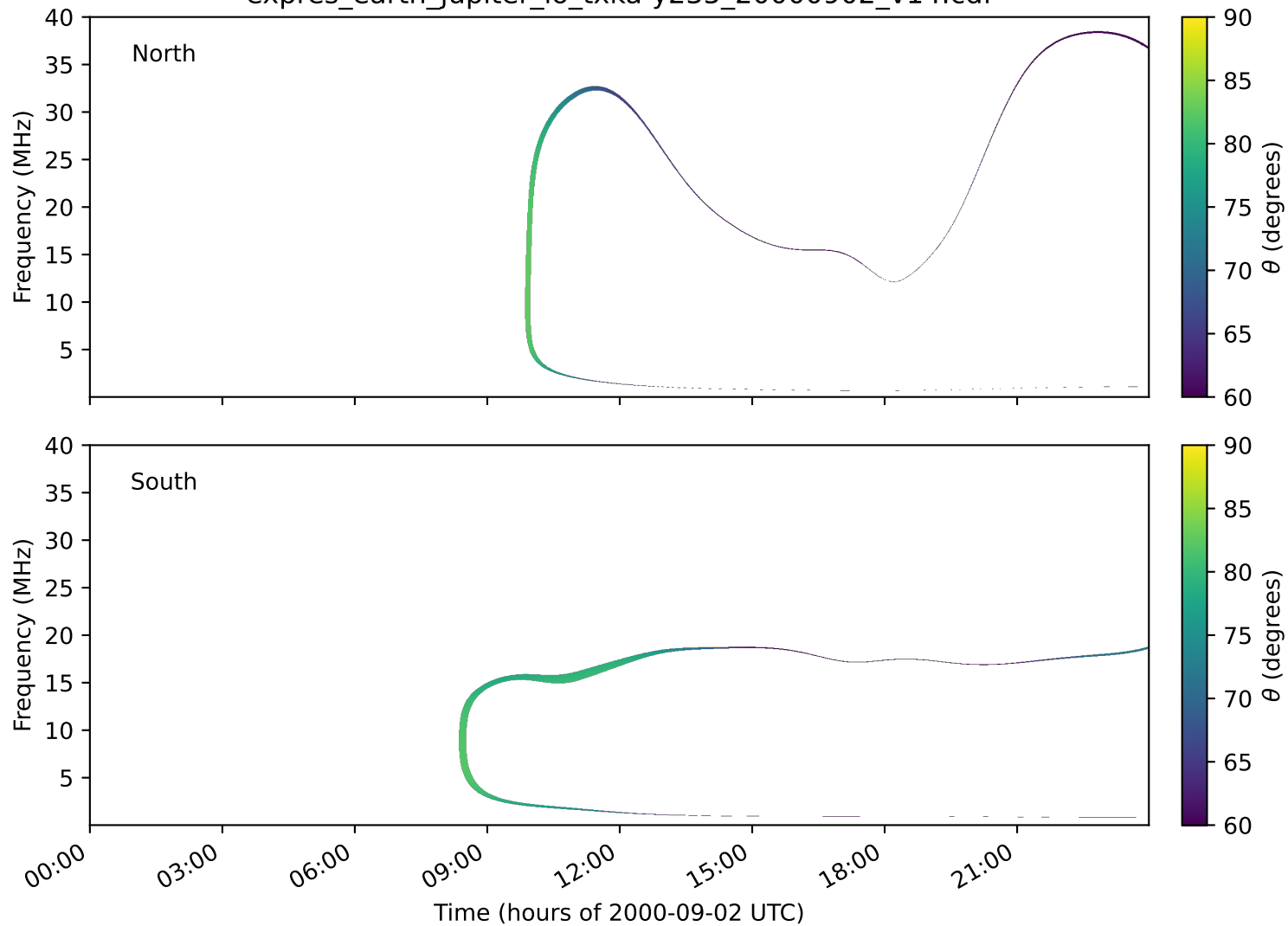
expres_earth_jupiter_io_txka-y235_20000902_v14.cdf
