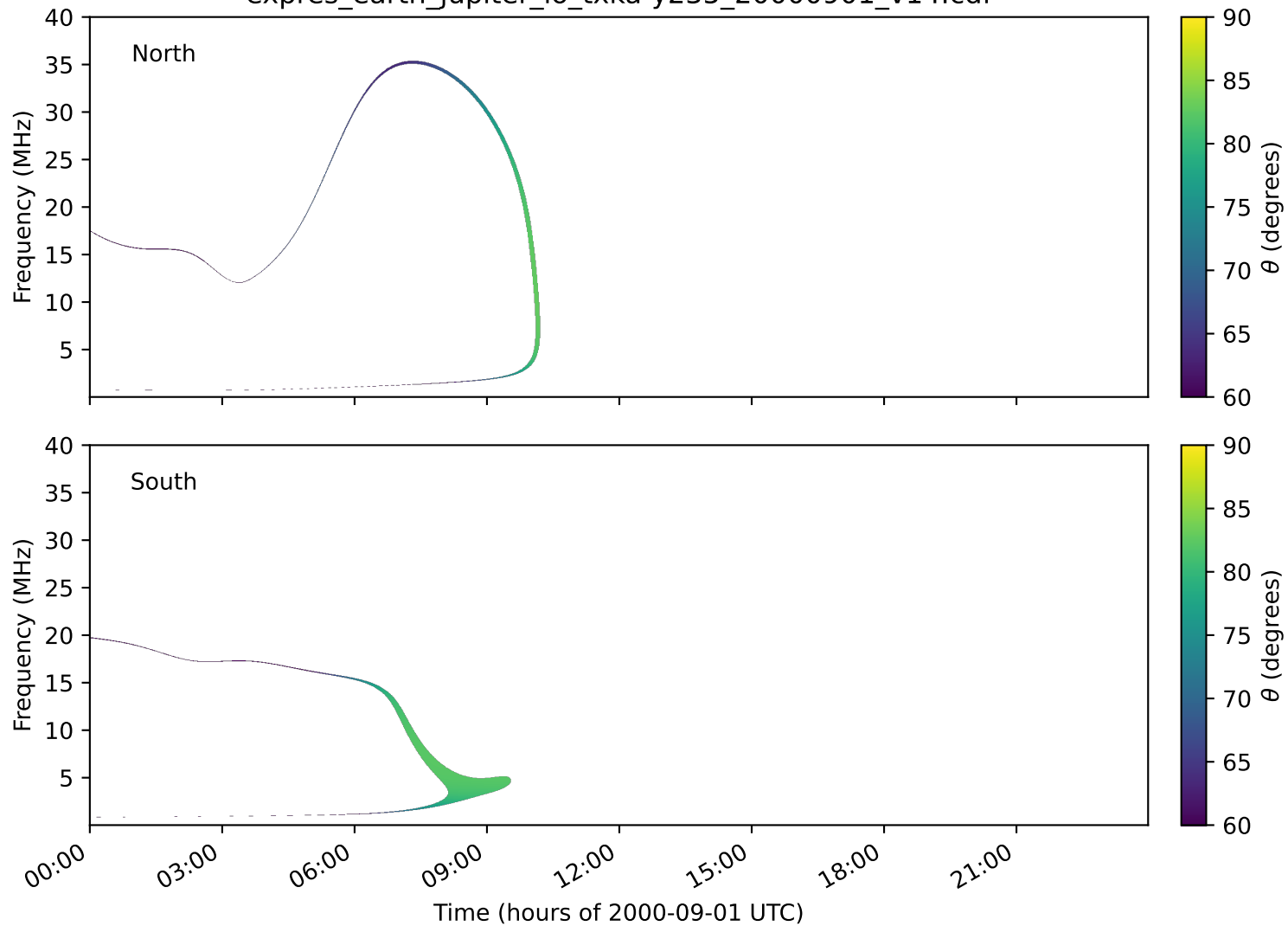
expres_earth_jupiter_io_txka-y235_20000901_v14.cdf
