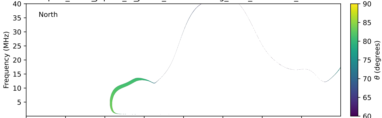
expres_earth_jupiter_io_jrm33_lossc-wid1deg_3kev_20000918_v11.cdf
