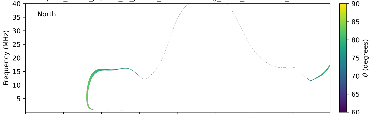
expres_earth_jupiter_io_jrm33_lossc-wid1deg_3kev_20000911_v11.cdf
