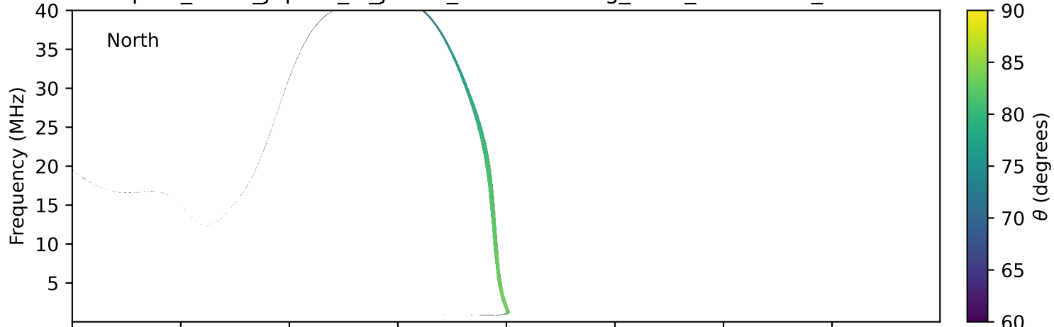
expres_earth_jupiter_io_jrm33_lossc-wid1deg_3kev_20000908_v11.cdf
