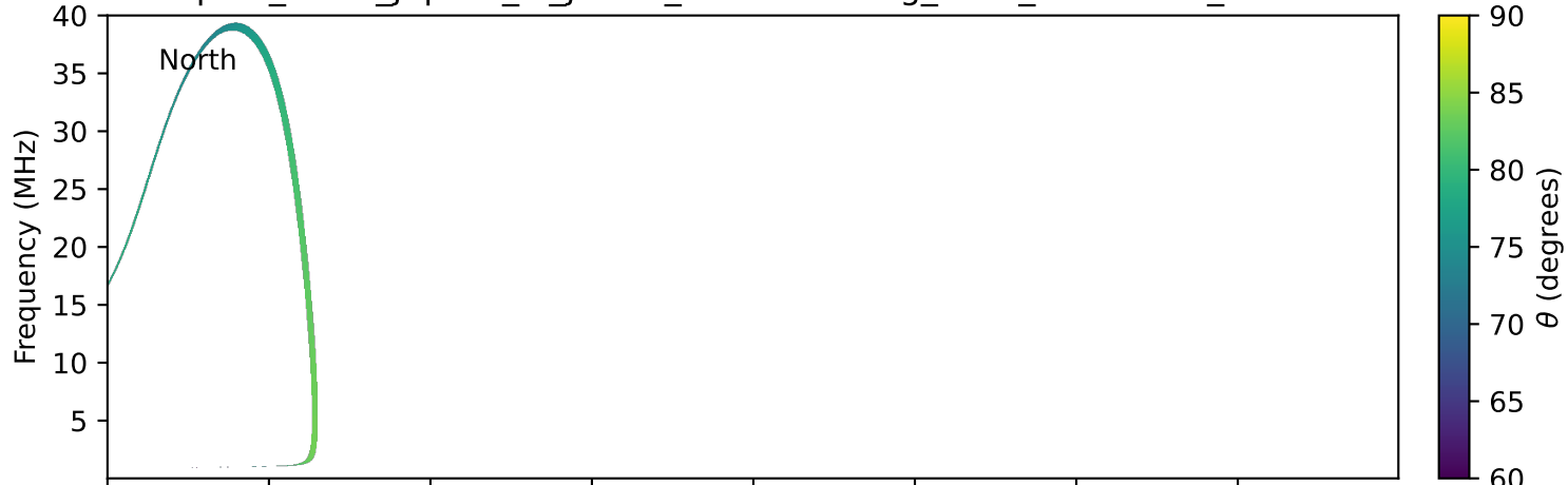
expres_earth_jupiter_io_jrm09_lossc-wid1deg_3kev_20000919_v11.cdf
