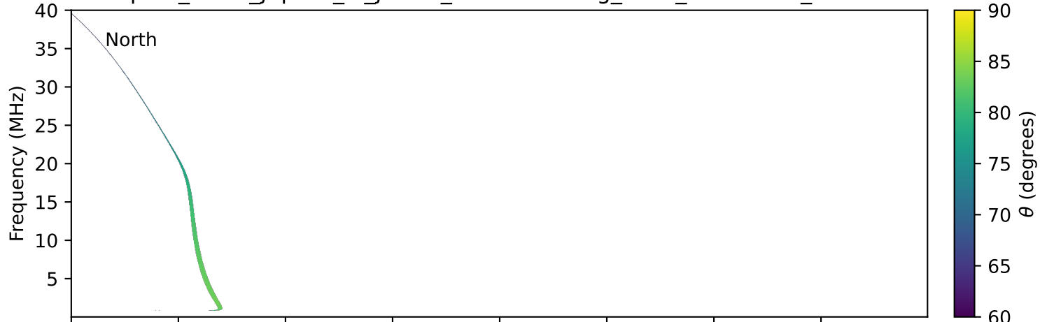
expres_earth_jupiter_io_jrm09_lossc-wid1deg_3kev_20000903_v11.cdf
