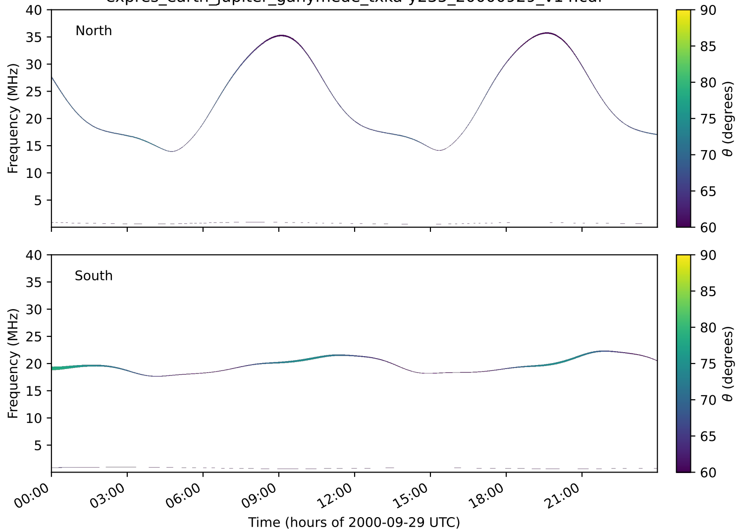
expres_earth_jupiter_ganymede_txka-y235_20000929_v14.cdf
