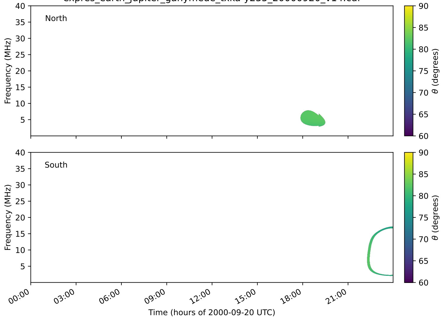
expres_earth_jupiter_ganymede_txka-y235_20000920_v14.cdf
