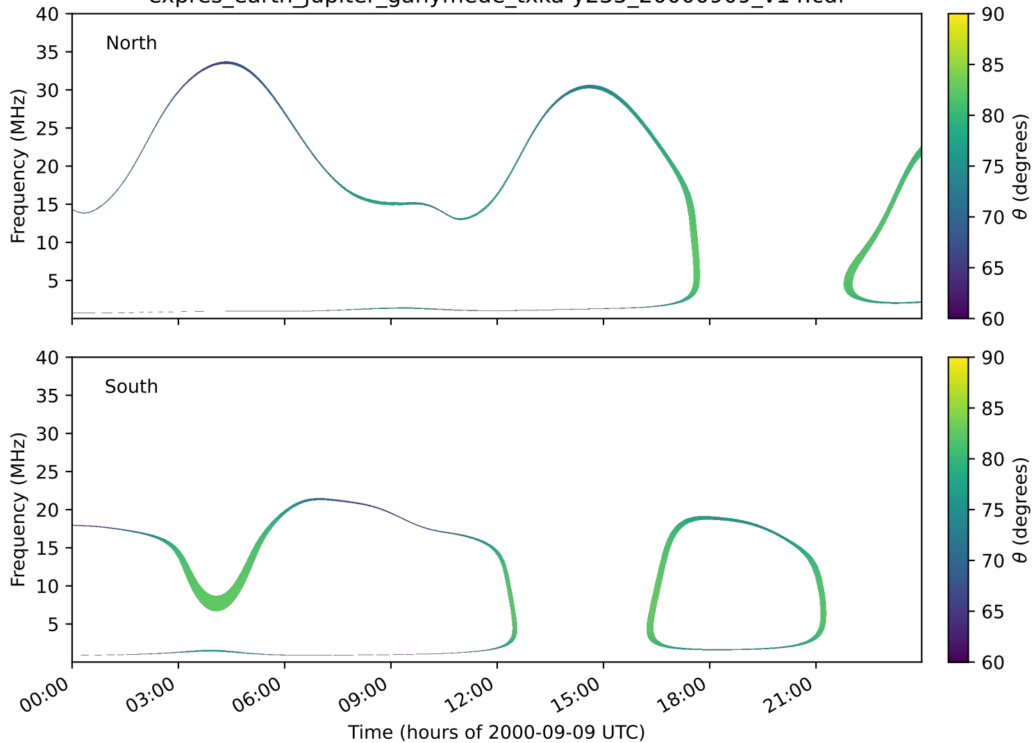
expres_earth_jupiter_ganymede_txka-y235_20000909_v14.cdf
