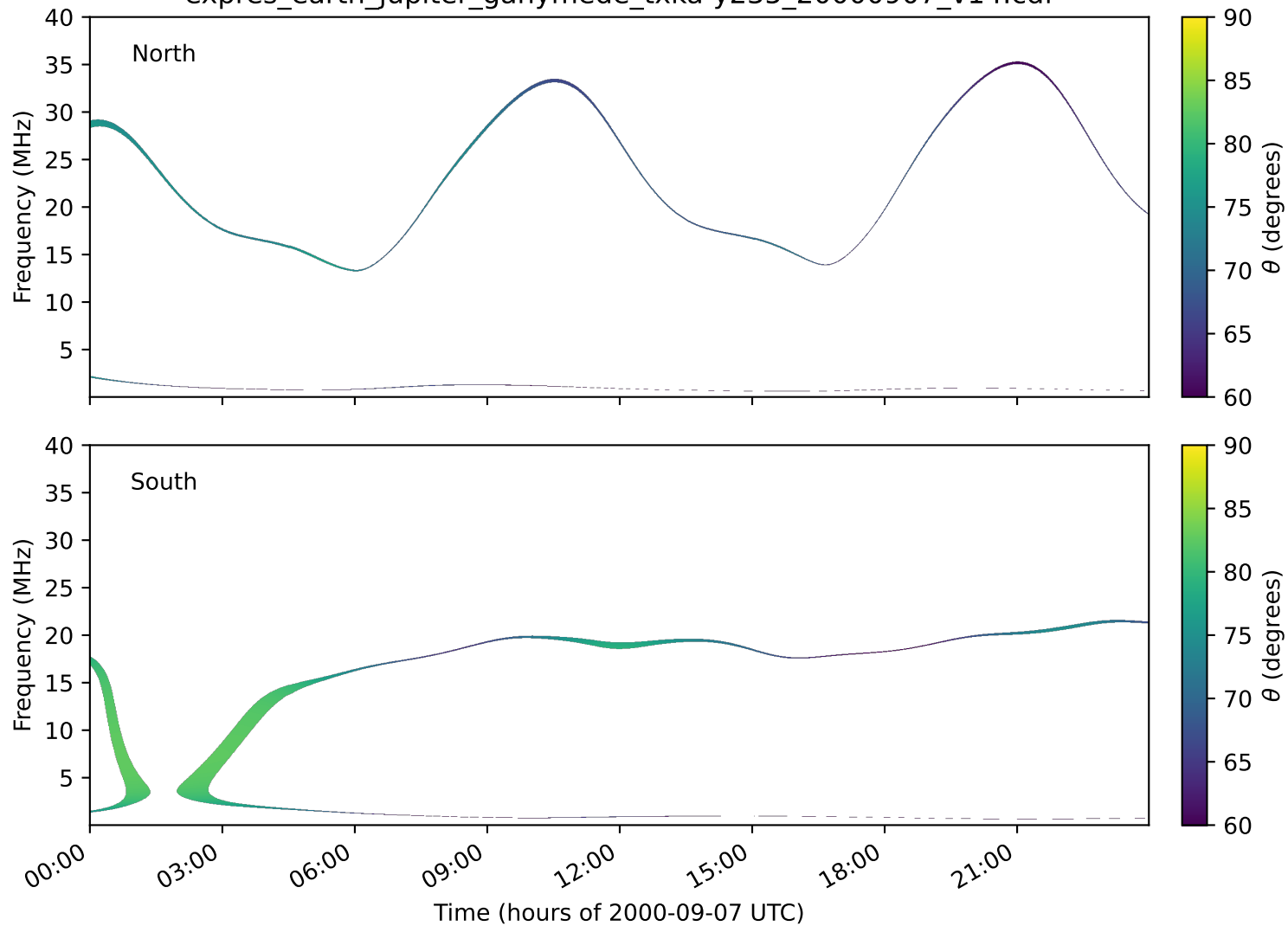
expres_earth_jupiter_ganymede_txka-y235_20000907_v14.cdf
